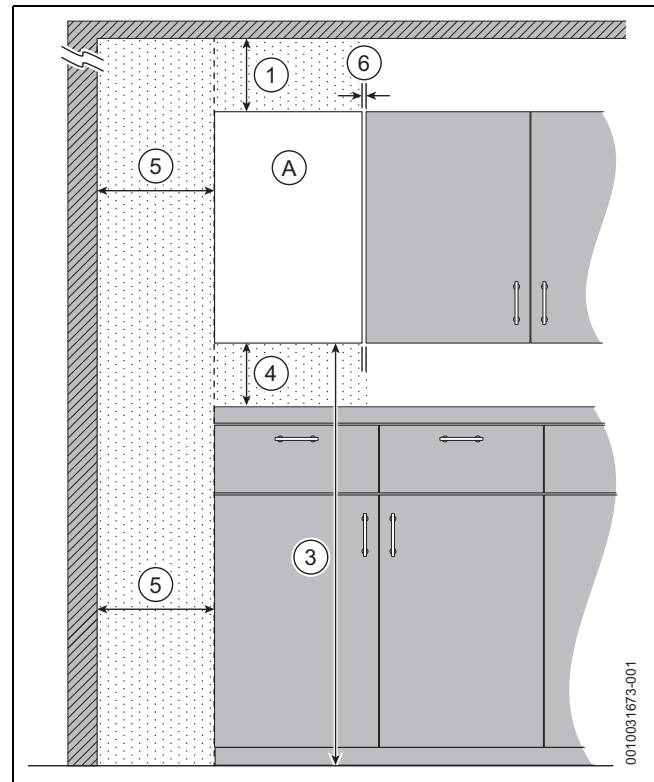
Fig. 9 Reduced front maintenance clearances - Front view
